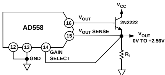
b. Output Current Booster Figure 8. Use of V_{OUT} Sense
