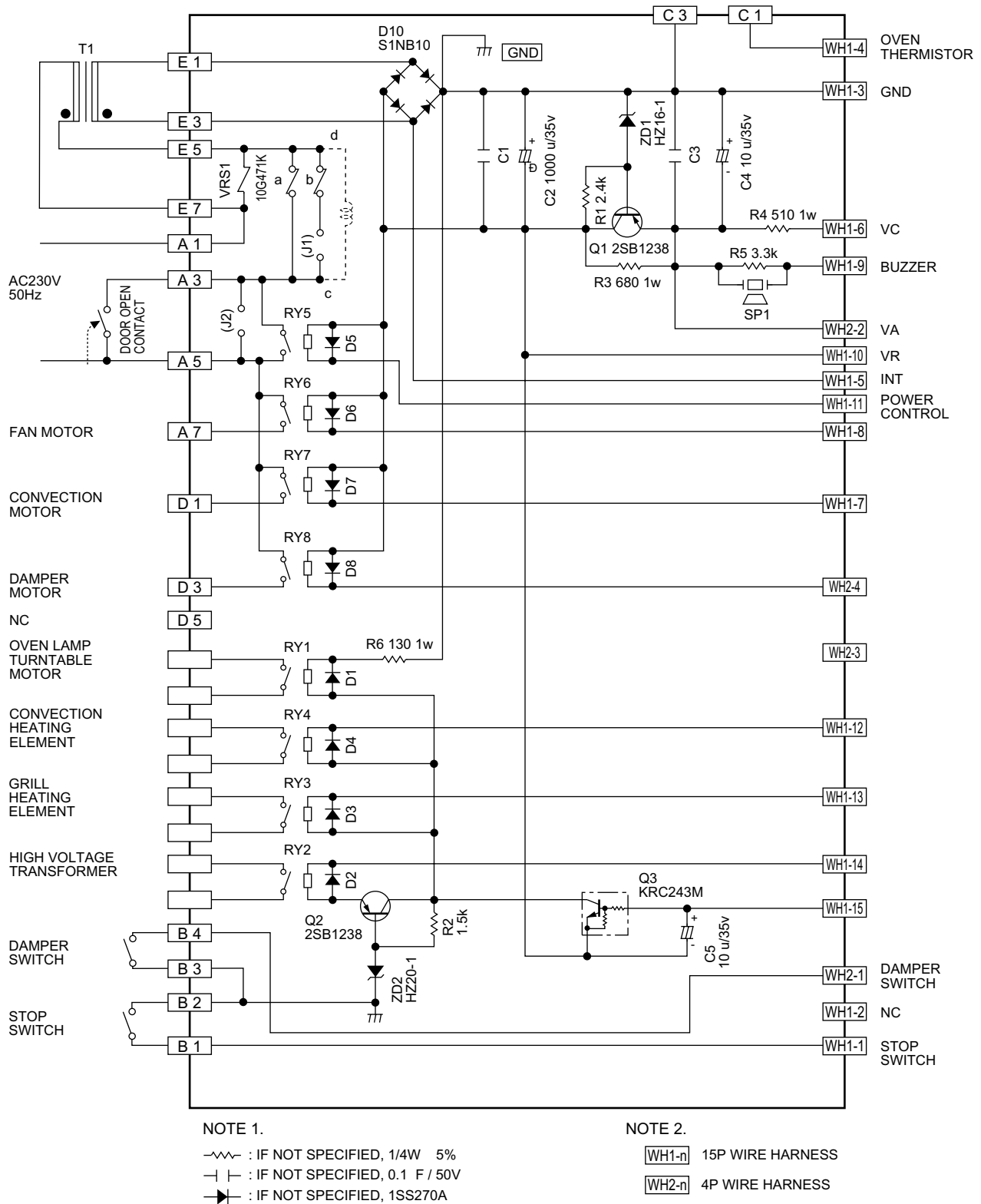
Figure S-2. Power Unit Circuit
