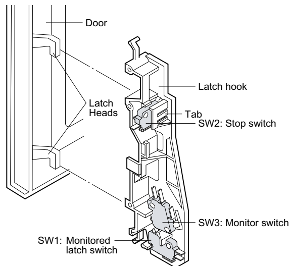
Figure C-6 Latch Switches Adjustment
