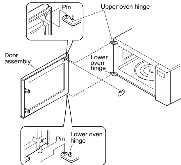
Figure C-8. Door Replacement
