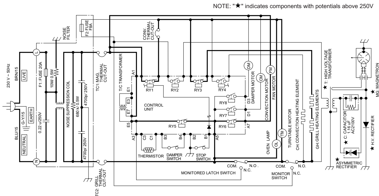
Figure O-3 Oven Schematic-Grill cooking Condition (TOP GRILL mode)
