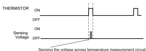
Sensing the voltage across temperature measurement circuit.
