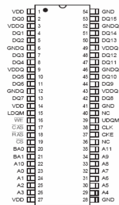
IS42S16400B-6TL;SDRAM (TSSOP-54)
