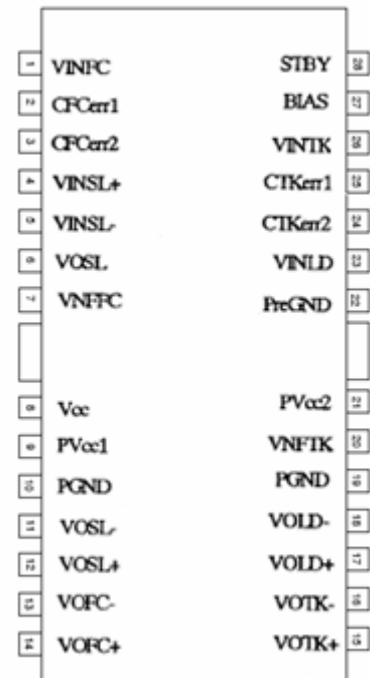
BA5888FP; Actuator driver (HSOP-28)
