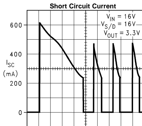
200 \text{ms}/\text{Div} Figure 19.
