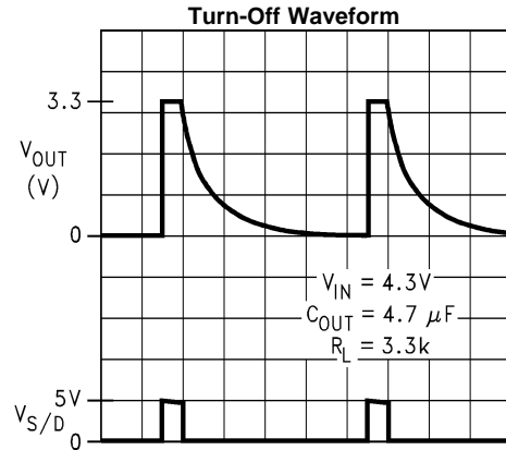
20 \text{ms}/\text{Div} Figure 17.
