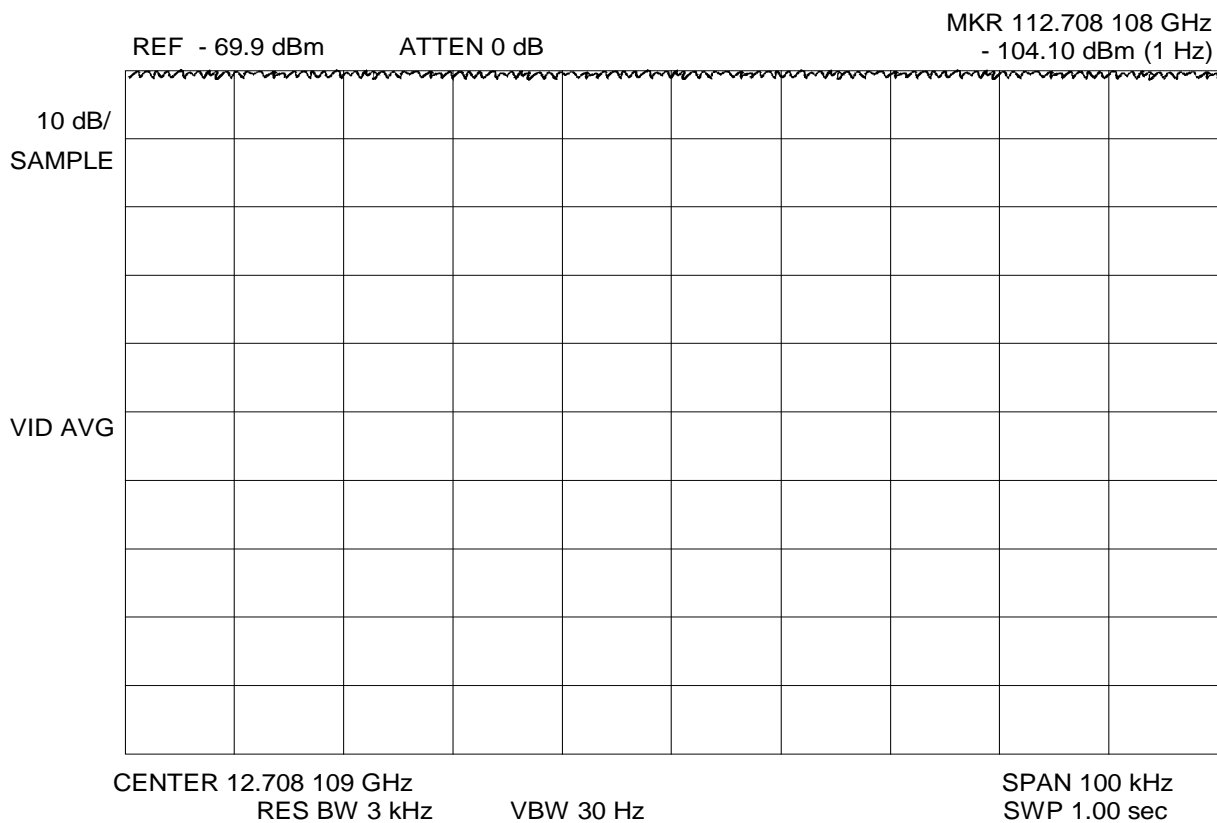
Figure 3 – Chapter 7: Spectrum Analyzer Display during G/T Measurement (Noise Level)
