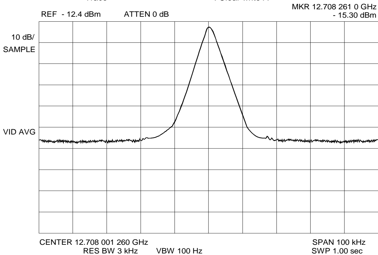
Figure 1 – Chapter 7: Spectrum Analyzer Display during G/T Measurement (Carrier Level)
