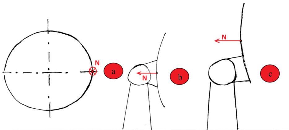
Figure 6 of Chapter 9: Yaw load certification;
