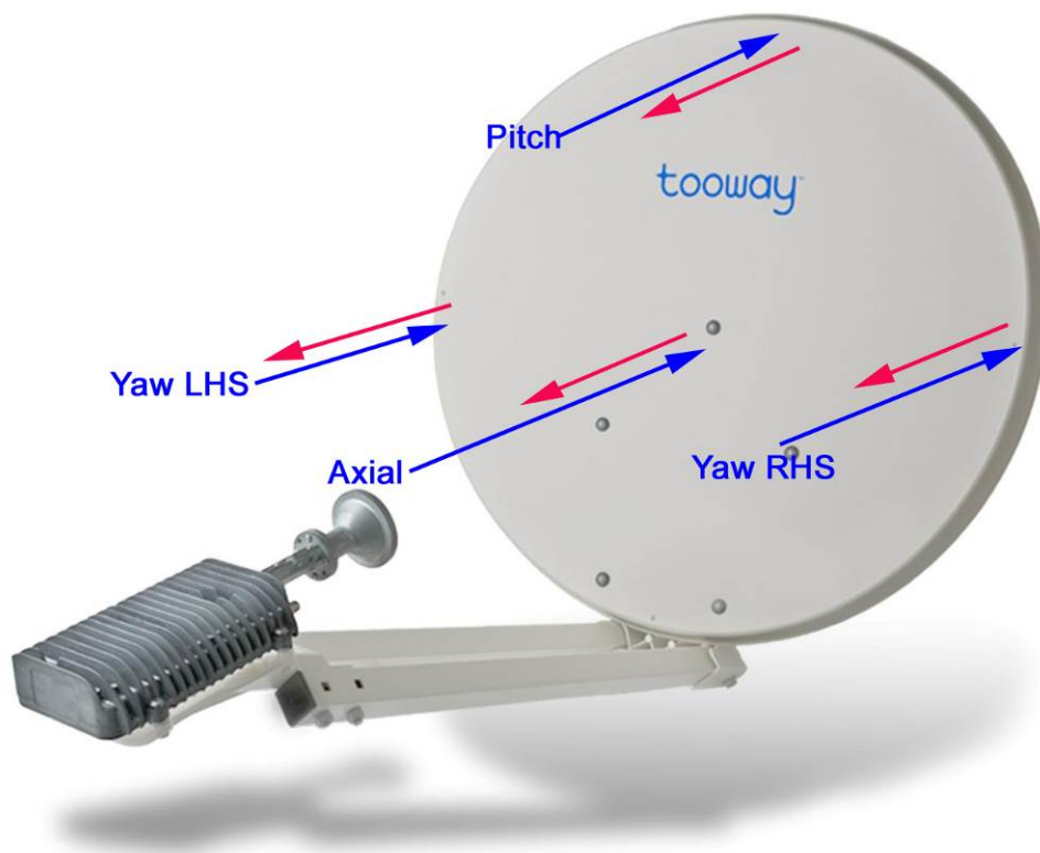
Figure 1 of Chapter 9 - Parabolic antenna forces, measured for wind load certification procedure
