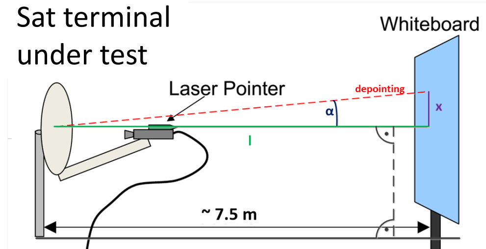
Figure 2 of Chapter 9 - Depointing test using a laser pointer
