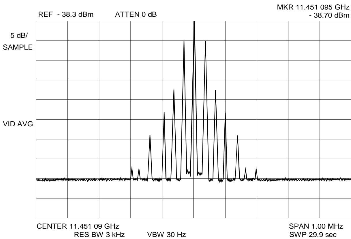
Figure 2 – Chapter 7: Spectrum Analyzer Display during G/T Measurement (Carrier Level)
