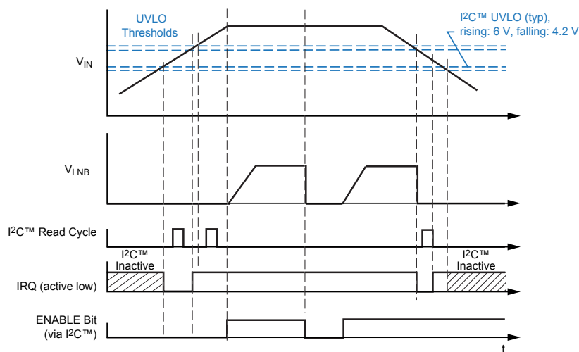
Figure 8. IRQ and Fault Clearing in Response to Undervoltage at V_{IN} (UVLO), the I^2C^{\text{TM}} port is active when V_{IN} is above I^2C^{\text{TM}} UVLO (6 V when V_{IN} is rising). IRQ transitions low when V_{IN} goes below I^2C^{\text{TM}} UVLO (4.2 V, V_{IN} falling), and the I^2C^{\text{TM}} Read cycle resets IRQ to logic high even if V_{IN} is below UVLO. Even though IRQ is cleared below UVLO, one more Read cycle is required after V_{IN} goes above UVLO, to re-enable the A8304. While V_{IN} is falling, IRQ transitions low when V_{IN} goes below UVLO, and the I^2C^{\text{TM}} Read cycle resets IRQ to logic high.
