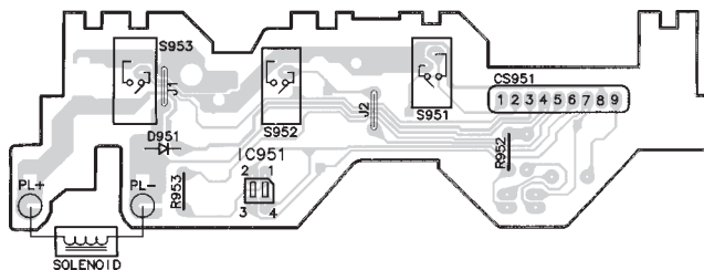
1 E MECHANISM (DECK 1) P.C.B. (REPX0108A)
