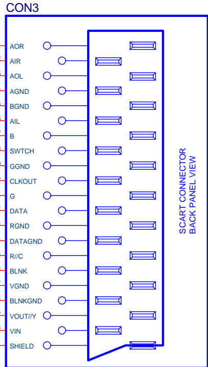
SCART CONNECTOR, RIGHT ANGLE, FEMALE
