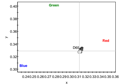
Chromacity Coordinates
