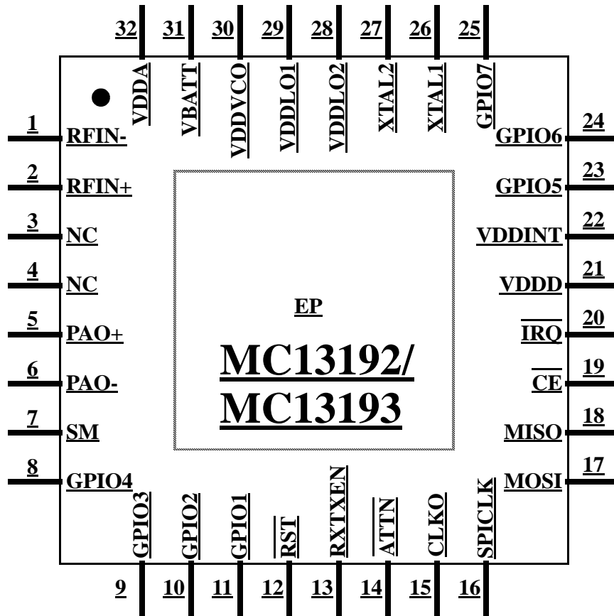
Figure 2-1. Device_Number Pinout
