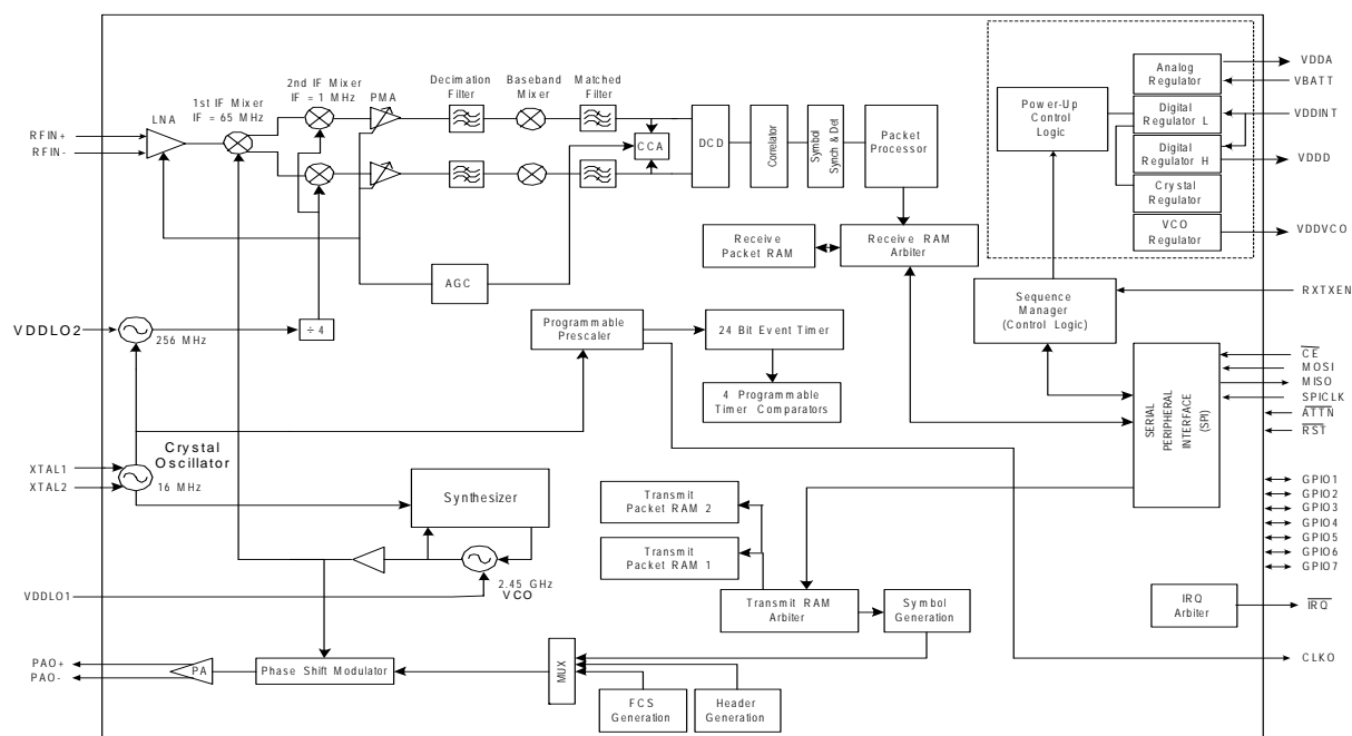
Figure 1-1. MC13192/93 Simplified Block Diagram
