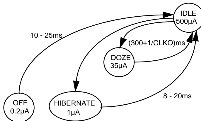
Figure 3-4. MC13192/MC13192 Modem Low Power Recovery Times
