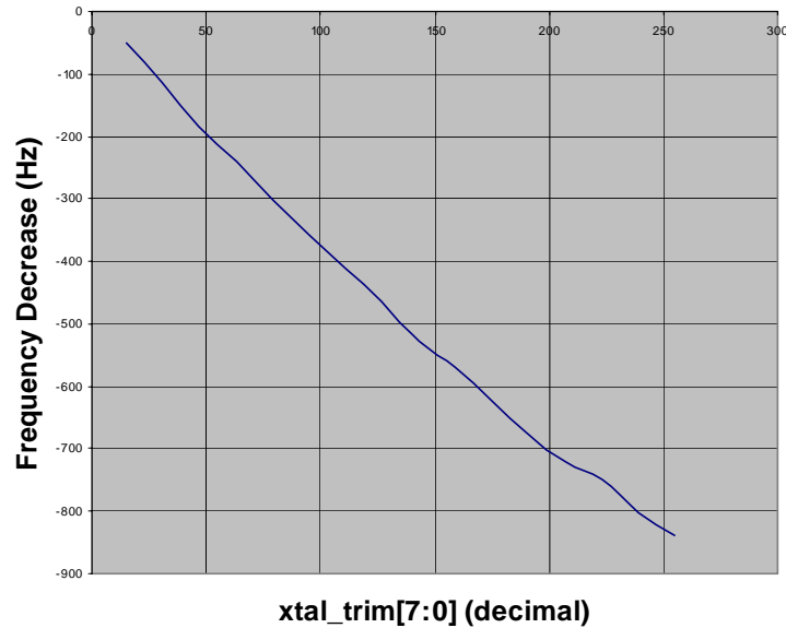
Figure 9-2. Crystal Frequency Variation vs. xtal_trim[7:0]
