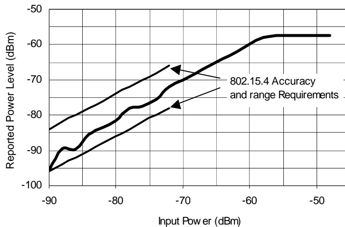
Figure 6-6. CCA Reported Power Level vs. Input Power
