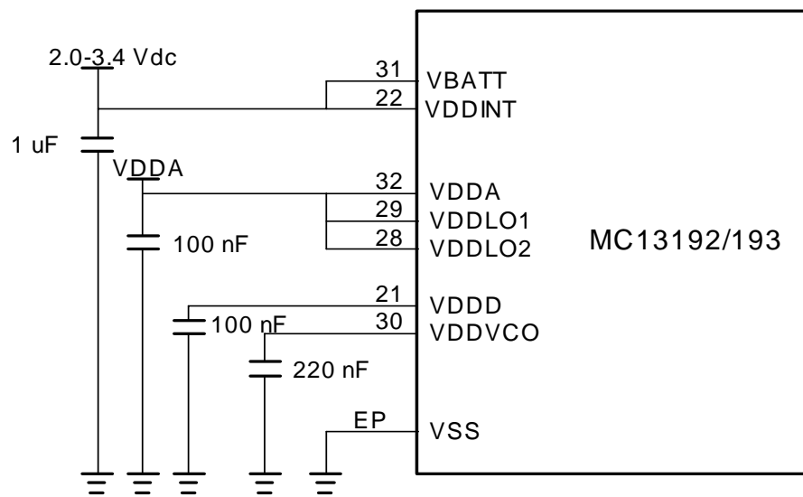
Figure 3-1. MC13192/193 Power Supply Connections
