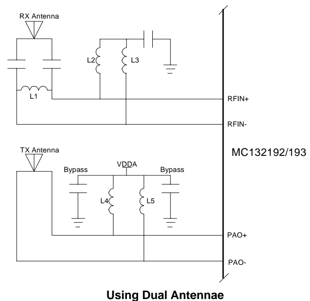
Figure 3-3. Dual Port RF Configuration Examples
