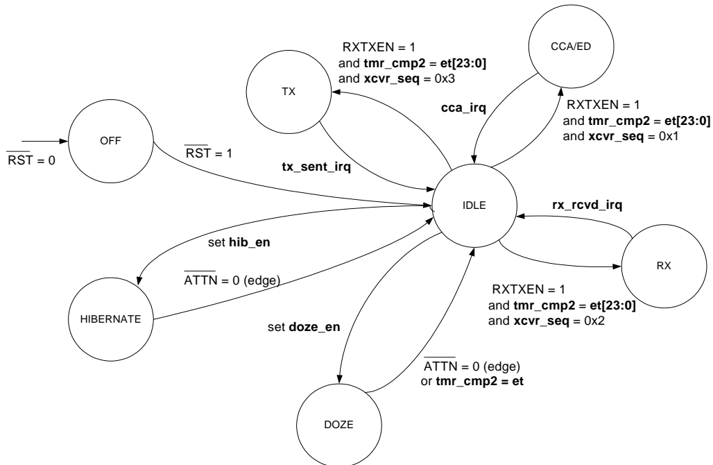
Figure 6-2. State Diagram for Packet Mode With Tmr_Cmp2 Enabled States ( tmr_trig_en = 1 )
