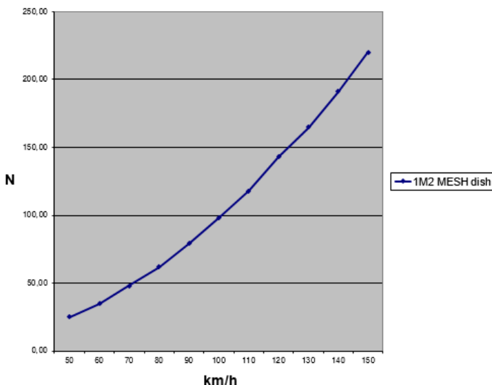
RF HAMDESIGN WIND LOAD - 1M2 MESH DISH 6mm Mesh
