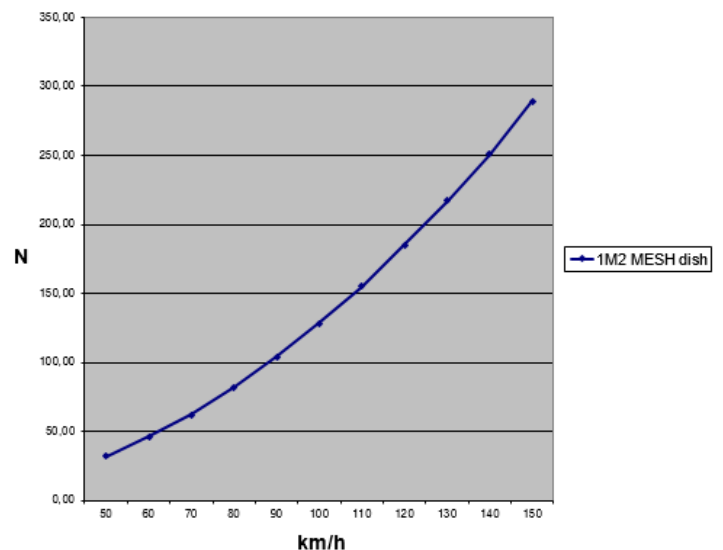
RF HAMDESIGN WIND LOAD - 1M2 MESH DISH 2.8mm Mesh
