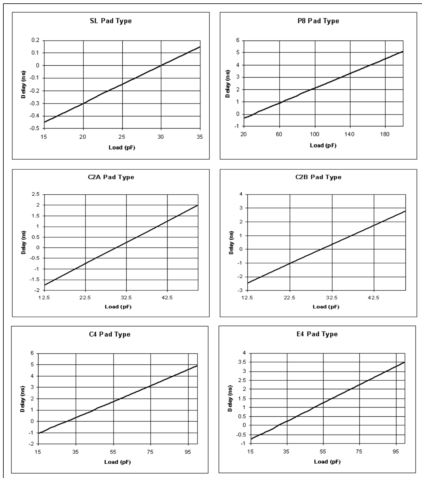
Figure 7: Pads characteristics
