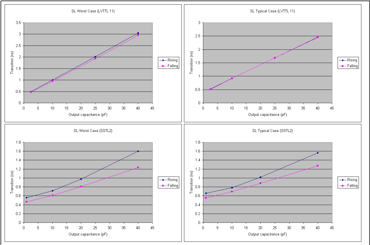
Figure 10: Timings for SL (LVTTTL 11 and SSTL2) pad types
