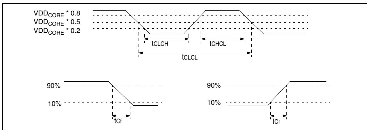
Figure 17: CLKIN timings
