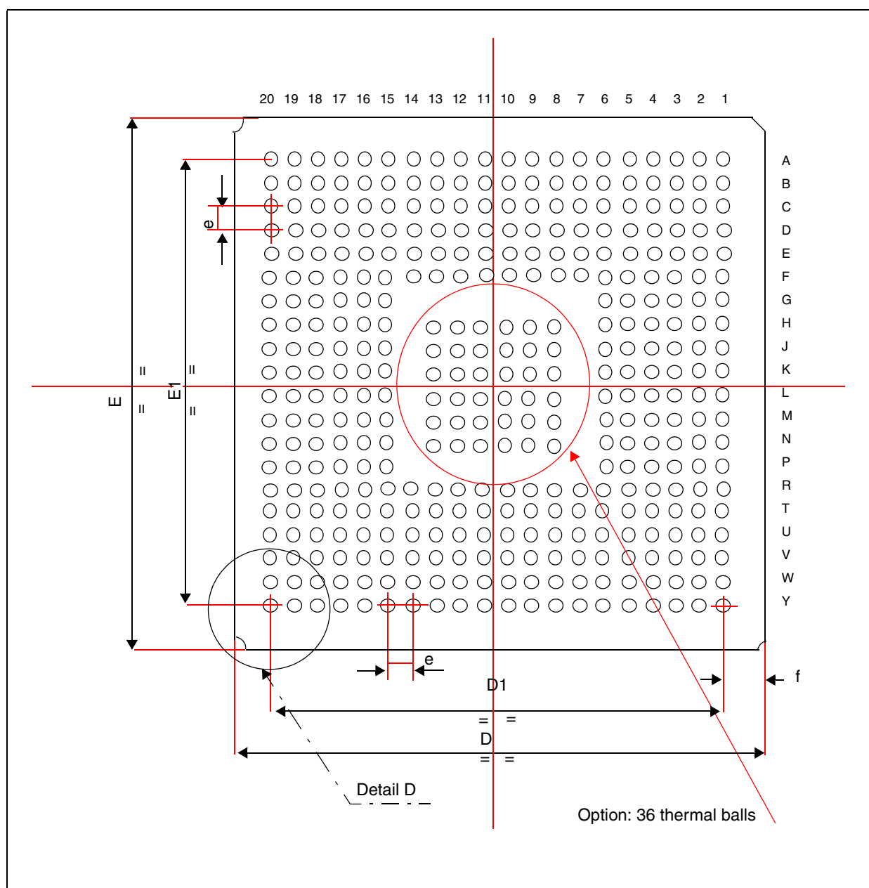
Figure 20: 372-pin PBGA package
