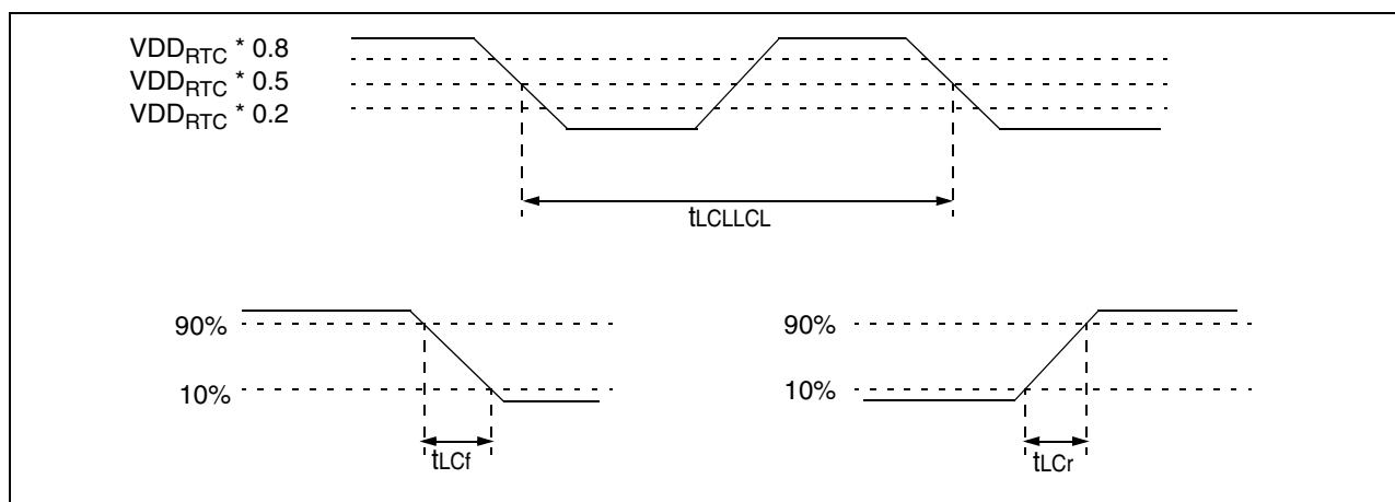
Figure 18: CLKIN timings
