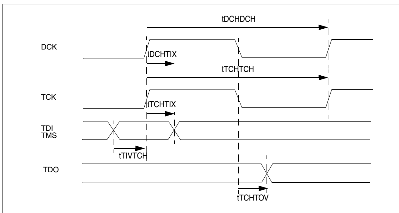
Figure 19: UDI and IEEE TAP timings
