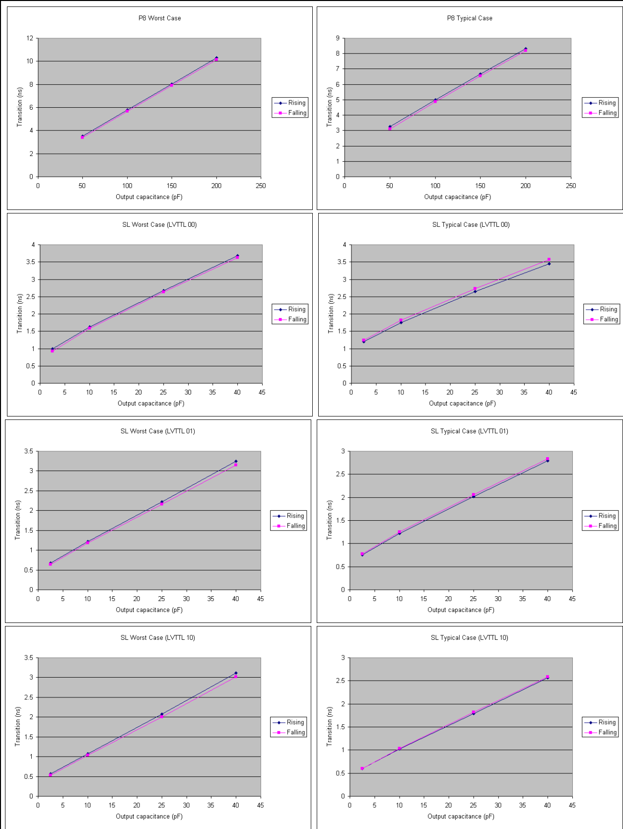
Figure 9: Timings for P8 and SL (LVTTL 00, 01 and 10) pad types
