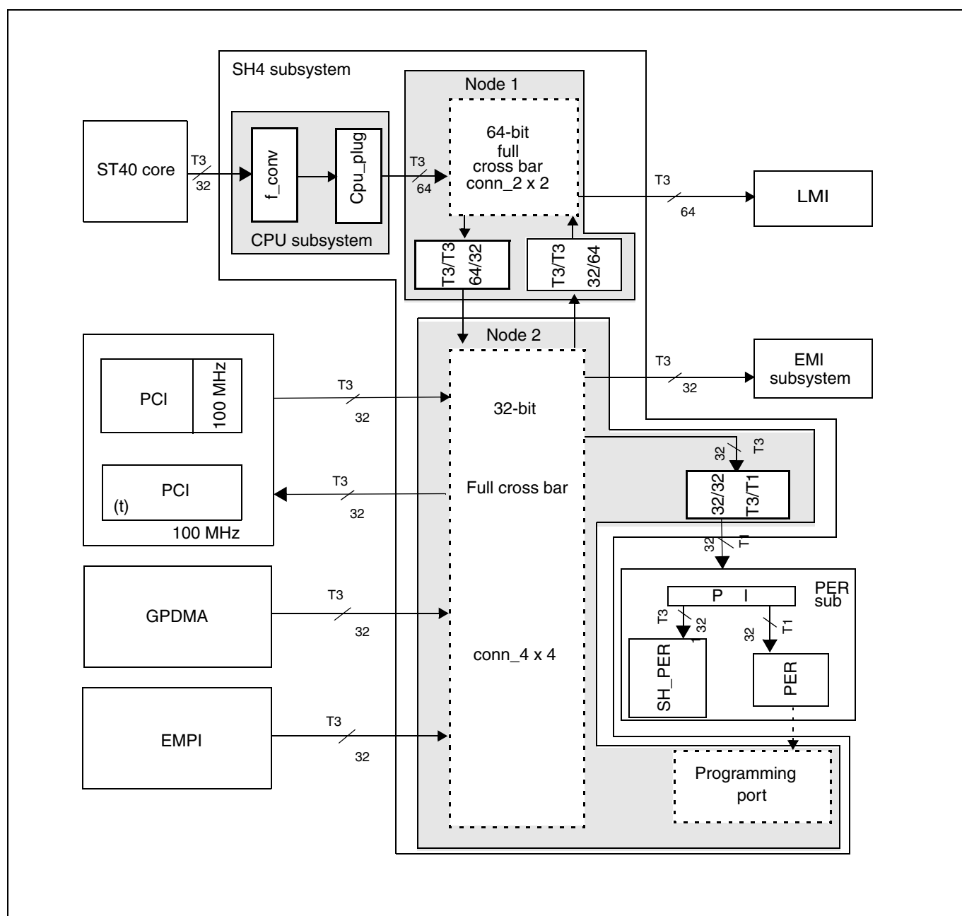
Figure 1: ST40RA interconnect architecture
