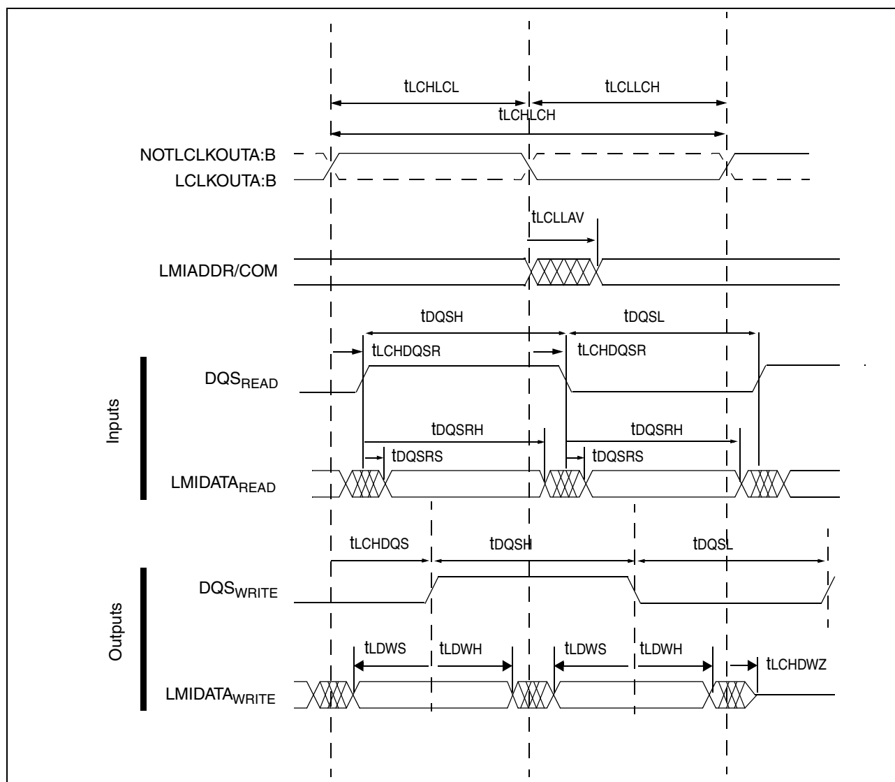
Figure 13: LMI DDR mode timings
