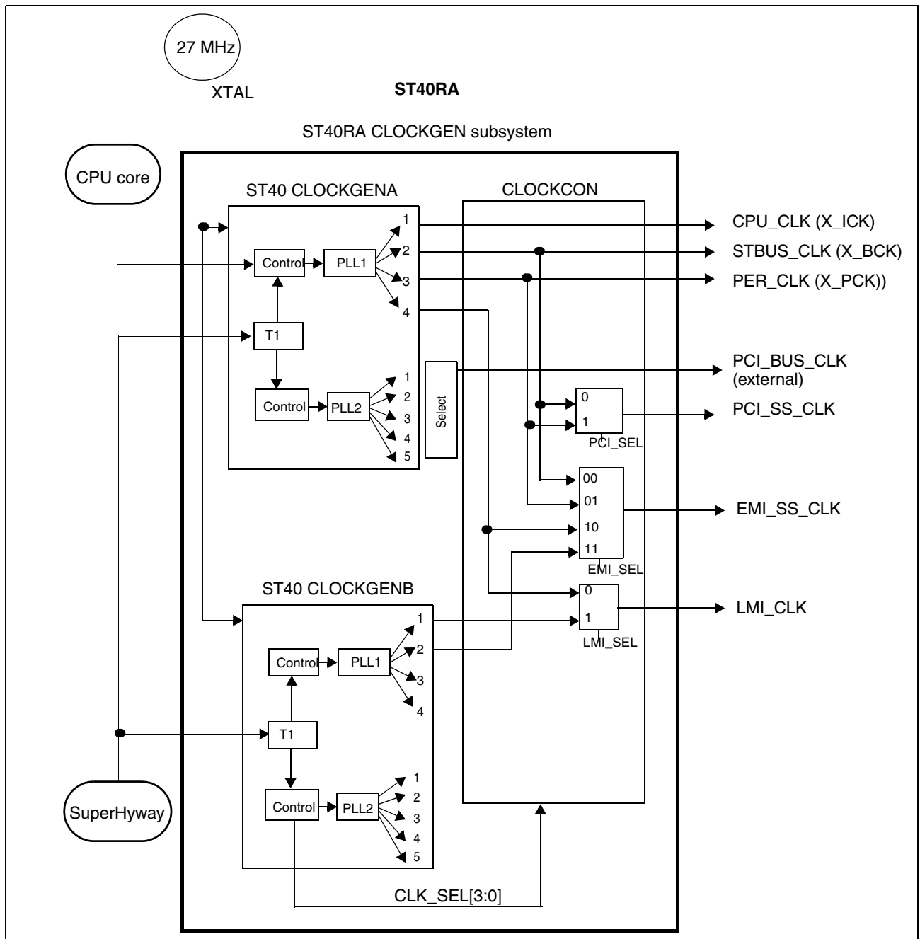
Figure 6: ST40RA CLOCKGEN subsystem
