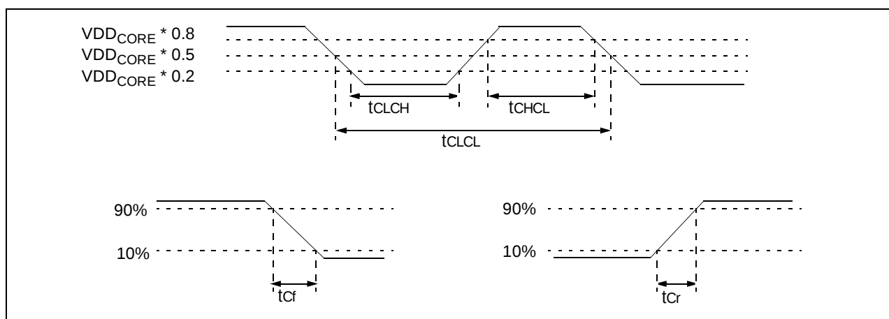
Figure 16: CLKIN timings
