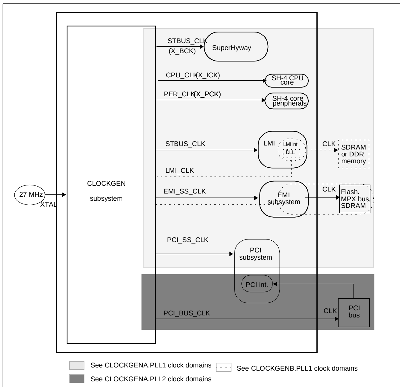
Figure 4: ST40RA clock domains
