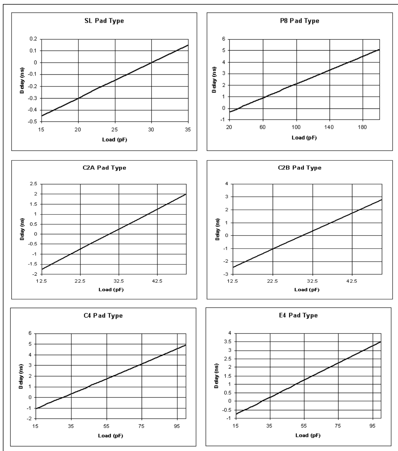
Figure 6: Pads characteristics
