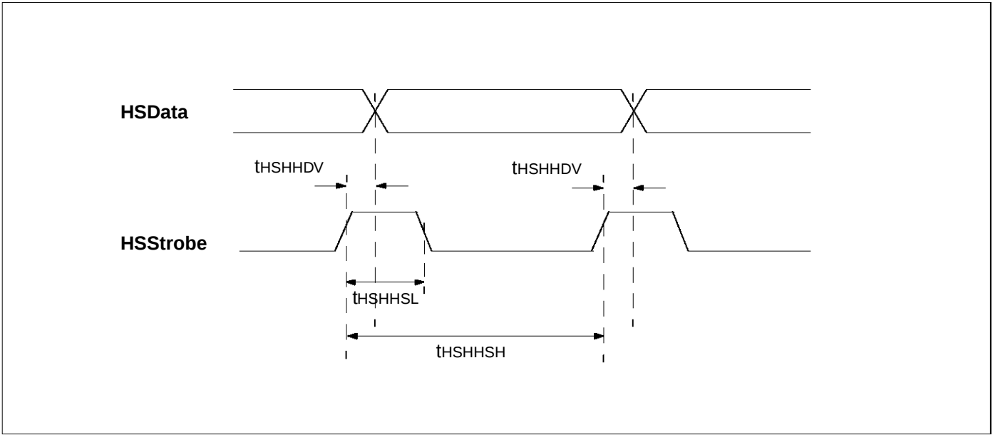
Figure 31.11 Data port timing diagram
