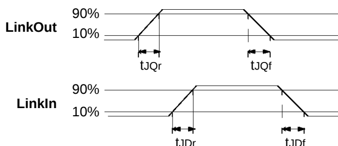
Figure 31.5 Link timings
