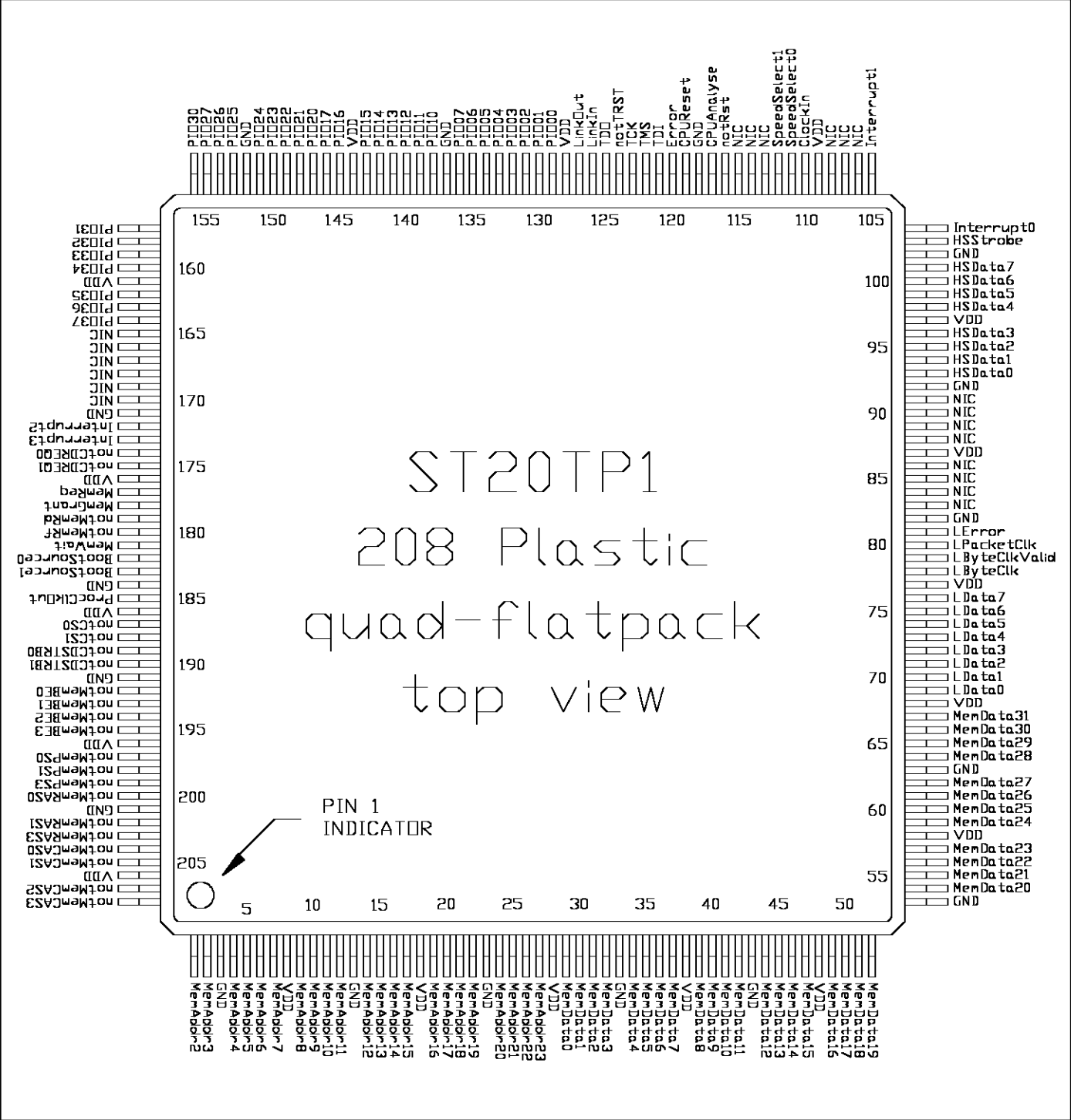
Figure 26.1 ST20-TP1 208 pin PQFP package pinout
