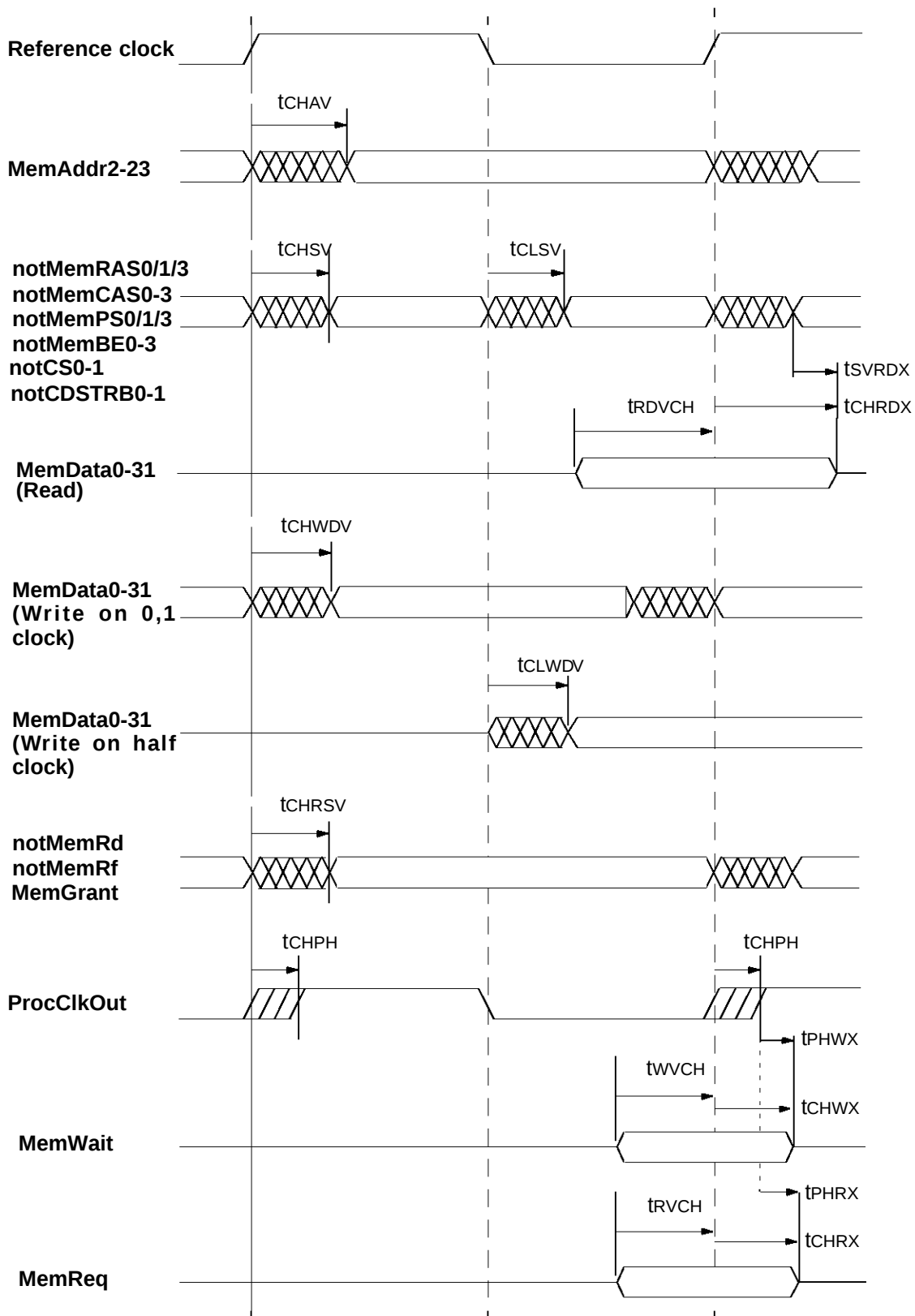
Figure 31.1 EMI timings
