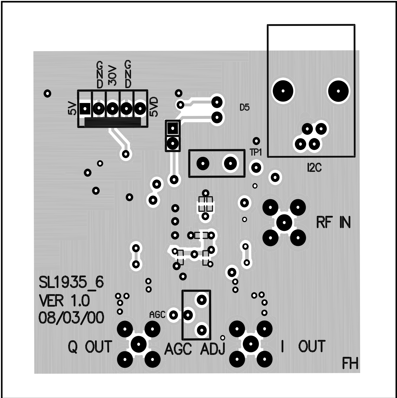
Figure 19. Top view
