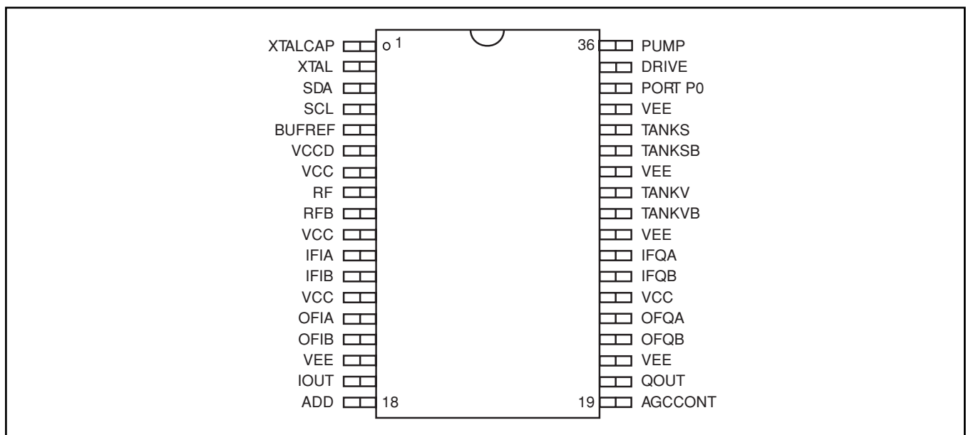
Figure 1. Pin connections
