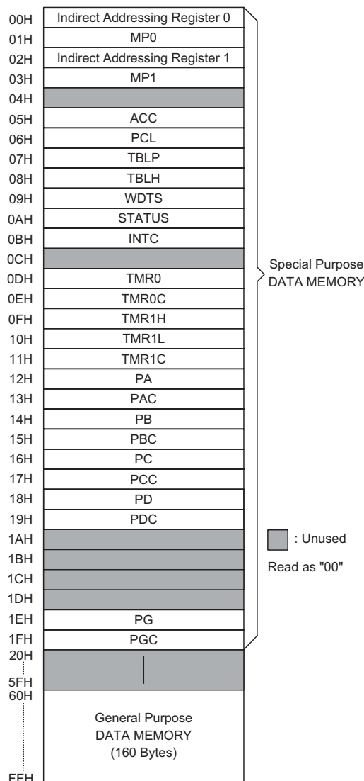
RAM Mapping
