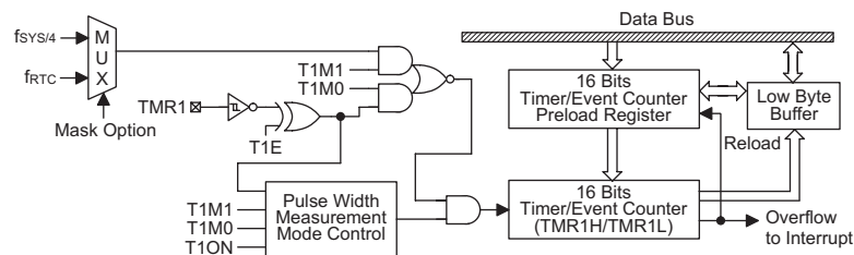
Timer/Event Counter 1
